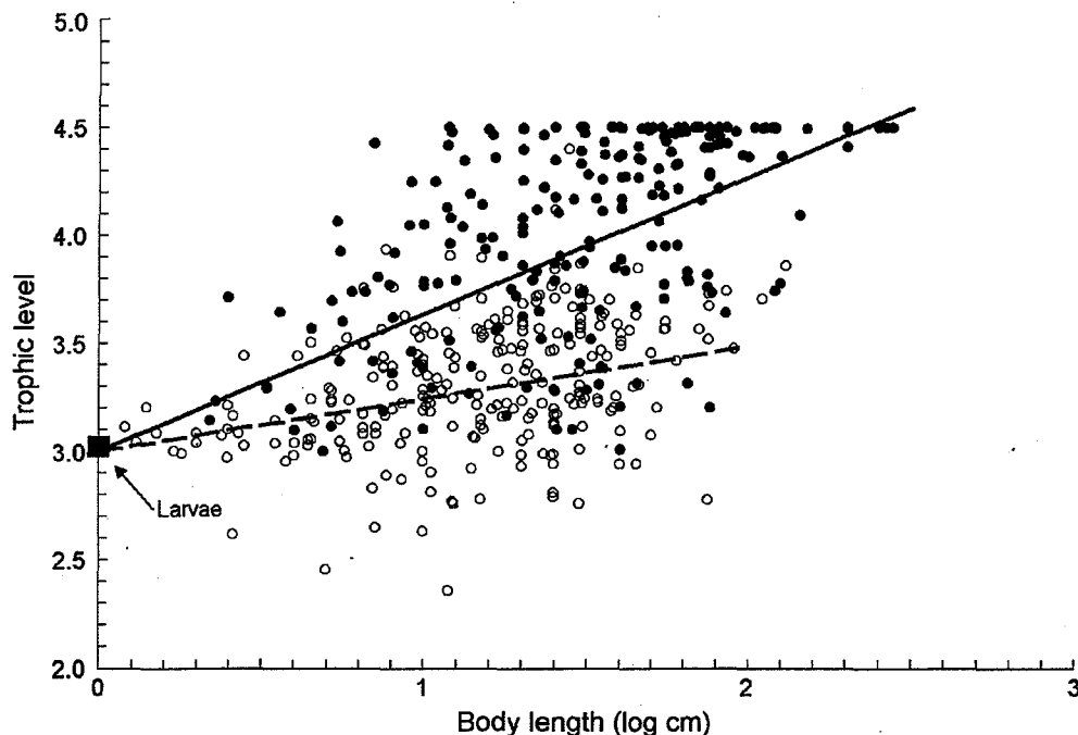
Fig. 1. Relationship between TL estimates and body length (cm) in 180 species of fishes. The regression lines (forced through the origin, representing larvae with TL = 3 and length ≈ 1 cm) have slopes of b_a = 0.24 for first-order carnivores (broken line and open circles, representing herring and other small pelagic and demersal fishes) and b_b = 0.63 for higher-order carnivores (solid line and solid circles, representing cod-like and other large piscivorous demersal and pelagic fishes).
